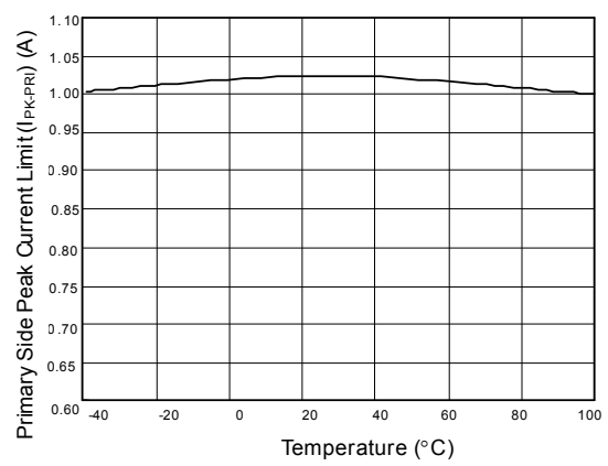
Fig. 14 Primary Side Peak Current Limit (R i =40kΩ)
